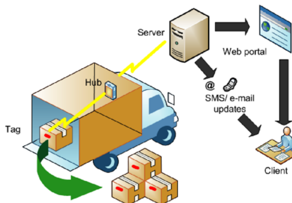
Figure 1. Conceptualization of an RFID system for monitoring cargo and air temperatures in a refrigerated transport system
